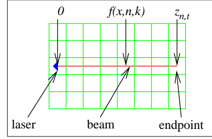
Figure 1: Beam covering z_{t,n} cells of a map.
